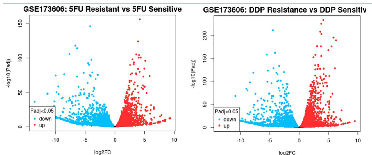
Figure 1. Tolcano plots of GSE173606 for acquired 5-Fu and DDP resistance COAD cells obtained from GEO2R analysis. X axis indicates the log2FC (or log2 fold change) of genes and Y axis is related to the adjusted P value which is the negative log10 of the adjusted P value. Red dots represent upregulated genes ( \log_2FC > 0 ) and blue dots represent downregulated genes ( \log_2FC < 0 ). In this study, genes with \log_2FC \geq 1 were considered high-expressed and genes with \log_2FC \leq -1 were considered low-expressed genes in chemoresistance cells.
